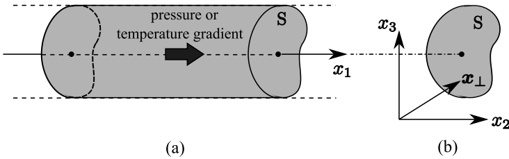
Fig. 2 Poiseuille and thermal transpiration flows. (a) Sketch of the problems. (b) Geometry of the pipe cross-section
